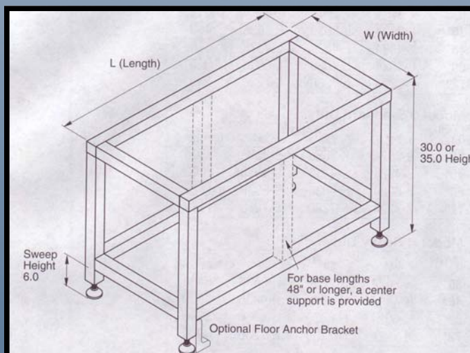
Standard Machine/Workstation Base
